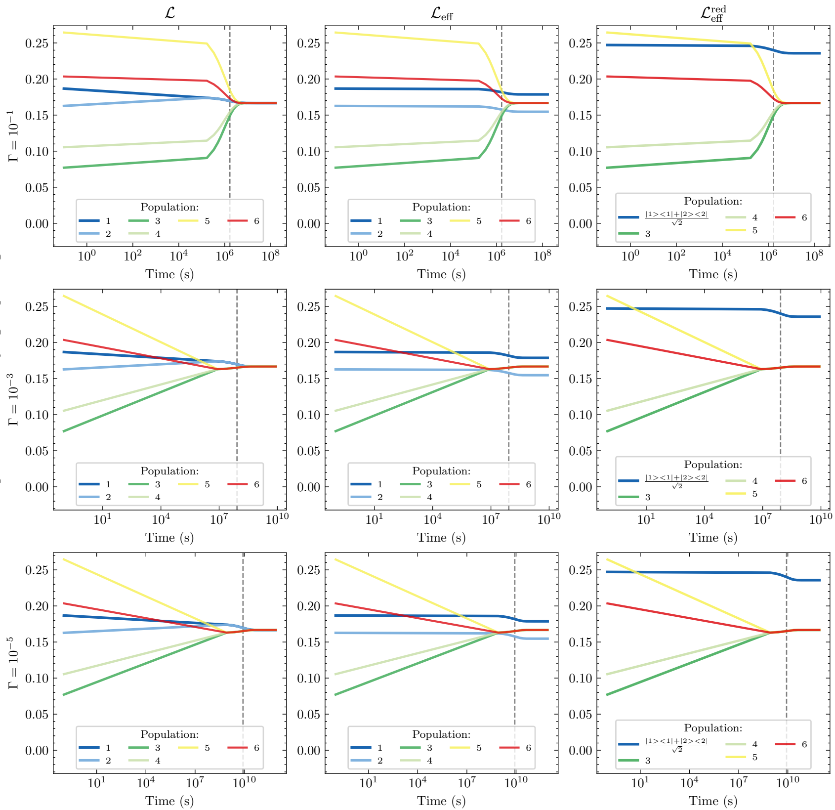
Time Evolution of Site Populations under \mathcal{L} , \mathcal{L}_{\text{eff}} , and \mathcal{L}_{\text{eff}}^{\text{red}} n=6 ; J = 10^{-1} ; \epsilon = 10^{-4}
